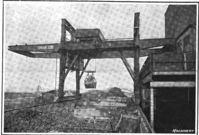
Fig. 31—This illustration shows a bin at the side of the railroad at the Ford Motor Co.'s plant in Detroit for storing coal, coke, limestone, scrap metal, etc. The Shaw Electric Crane Co., Muskegon, Mich., installed a gantry crane equipped with a grab bucket for handling this material
